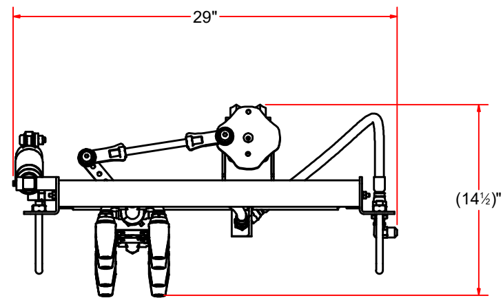
FRONT
