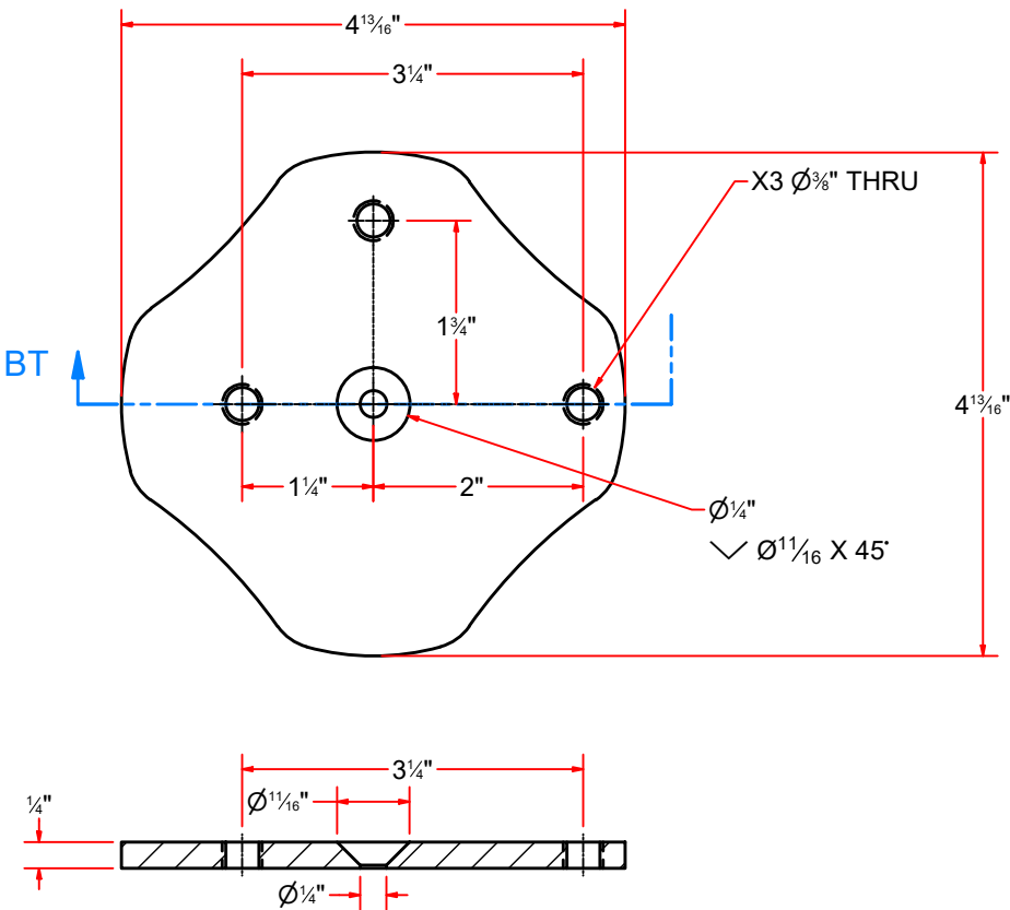
SECTION BT-BT
