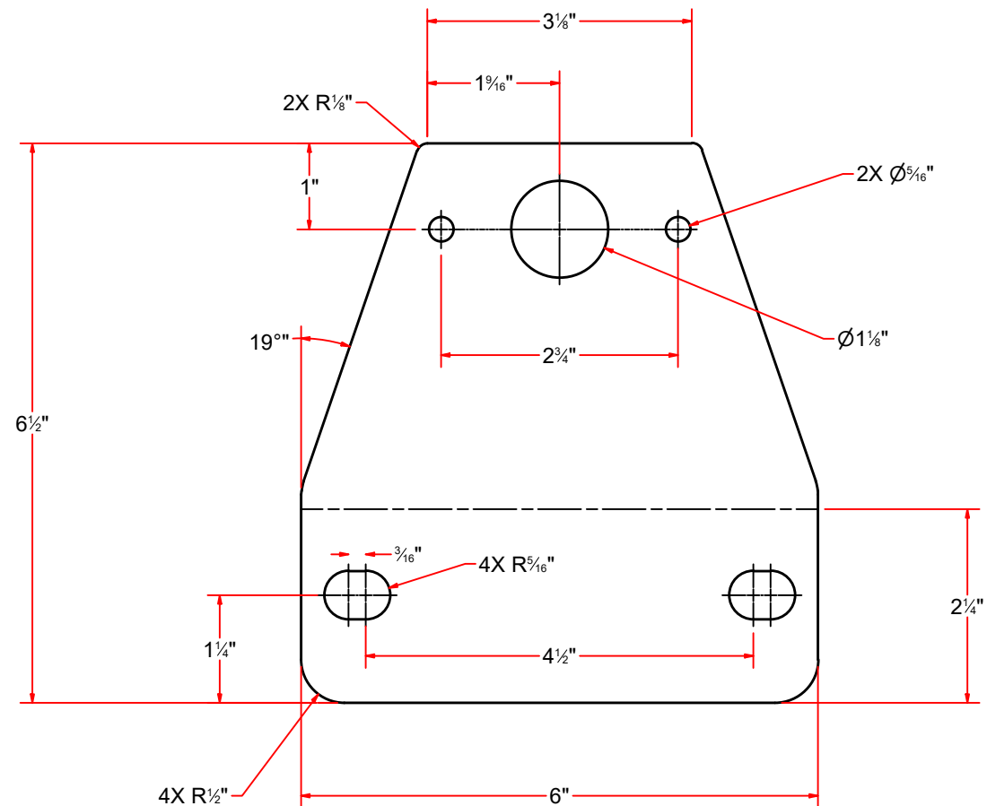
FLAT PATTERN
