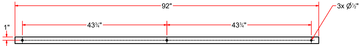
FRONT
