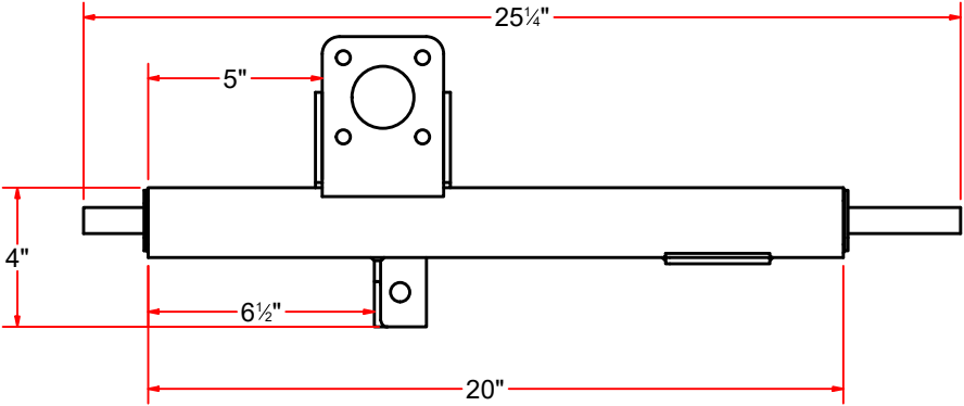
FRONT
