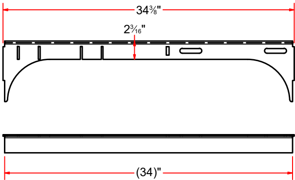
FORMED
