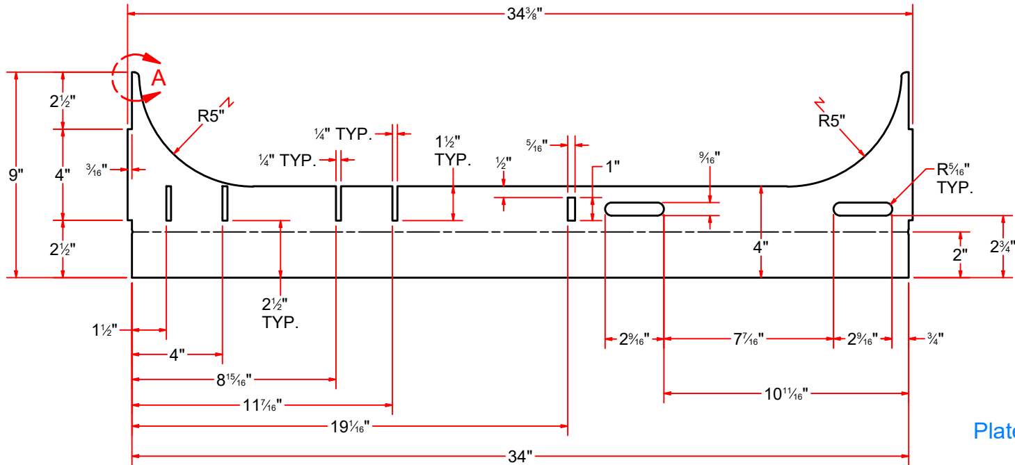
FORMED
