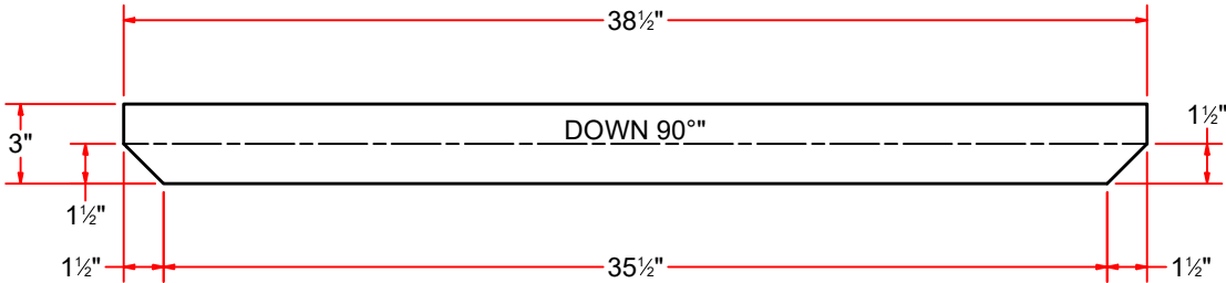
Angle #12Ga 1 1/2" x 1 1/2" x 38 1/2" LG.
