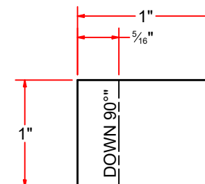
VIEW112
