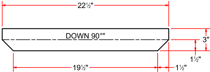
Angle #12Ga 1 1/2" x 1 1/2" x 22 1/2" LG.
