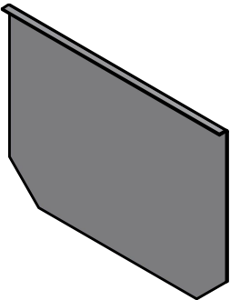
Baffle #12Ga (0.1046 in) x 17" x 22" LG.
