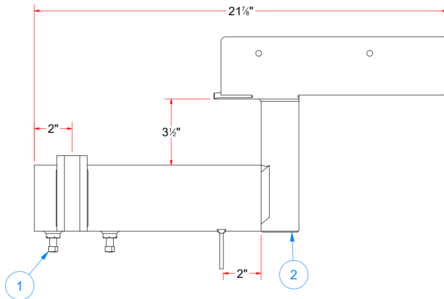
TB3BABA - Base Frame for Brush Drive Assembly [Passengerr - Hyd.]
