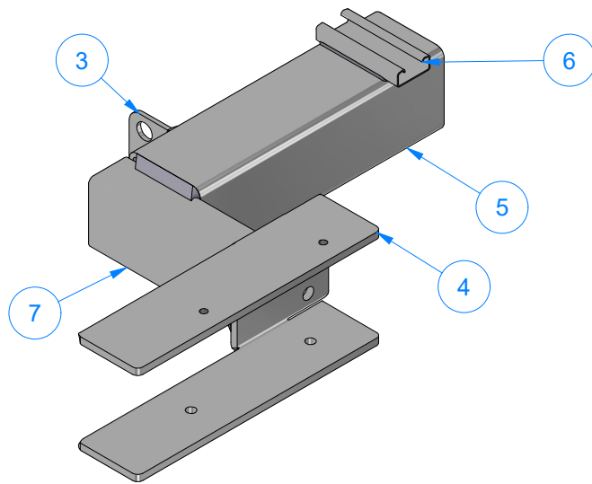
TB3BABA - Base Frame for Brush Drive Assembly [Passengerr - Hyd.]
