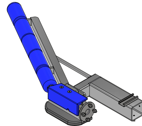
TB3AAA - Push Bar Assembly [Driver]
