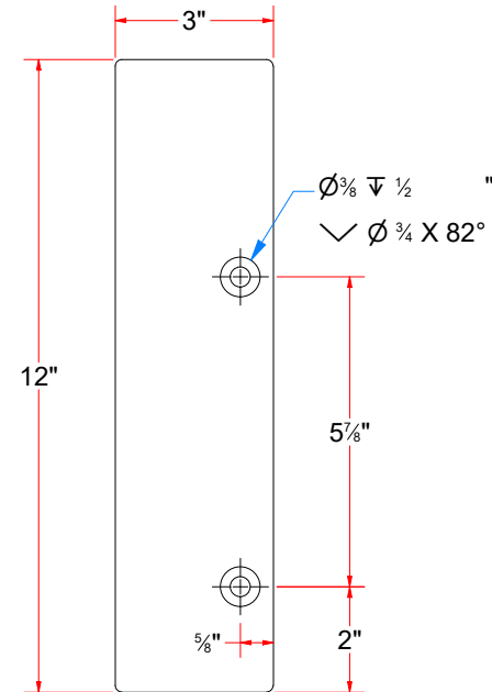
TB3BABB - Rear Exit Cover [Passenger]
