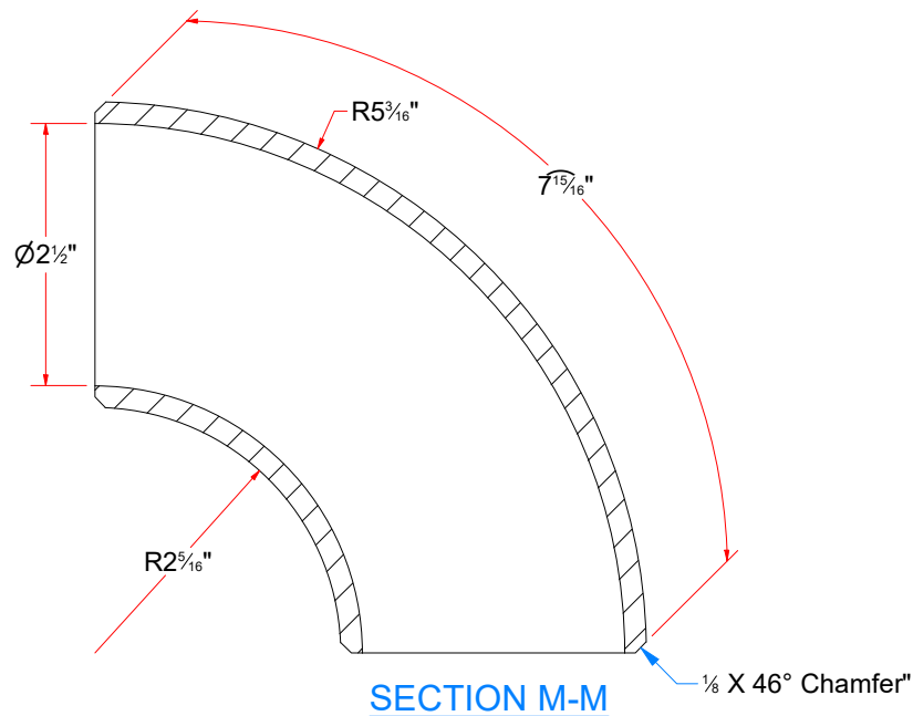
90 Deg Pipe Sweep Elbow - 2 1/2" Pipe Sch40
