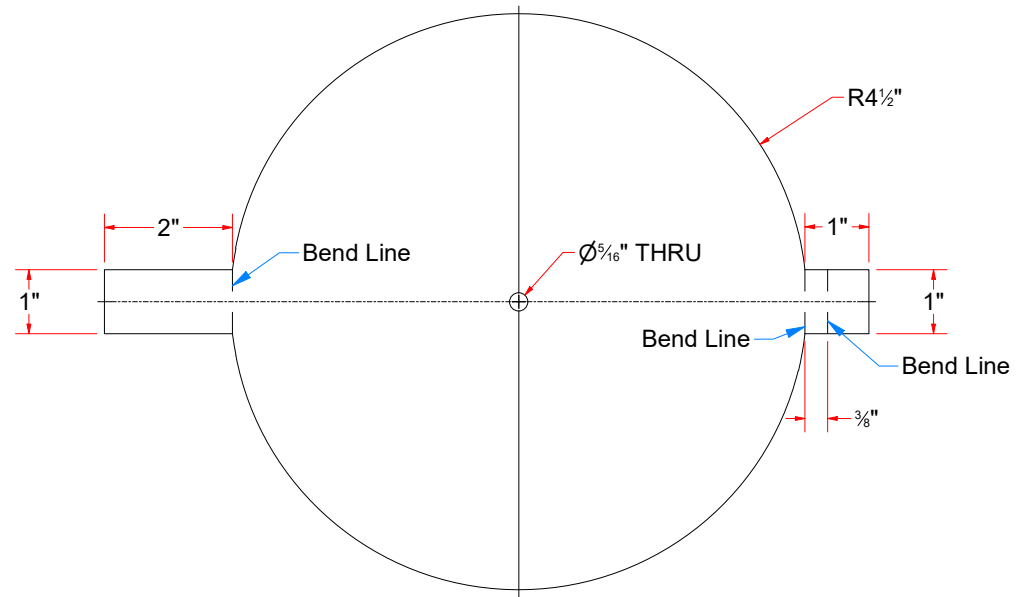
Flat Pattern
