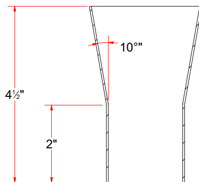
SECTION L-L
