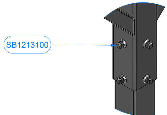
DETAIL B
