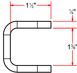
FORMED
