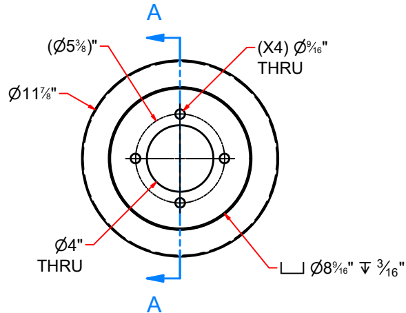
Alu. Plate #1/2" x 11-7/8"OD
