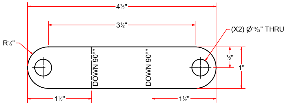
FLAT PATTERN
