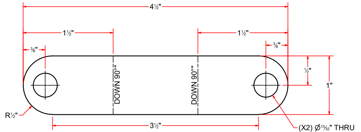
FLAT PATTERN
