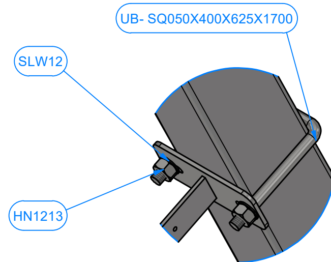
DETAIL M
