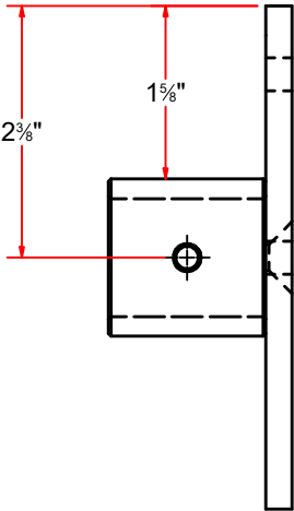
SIDE
