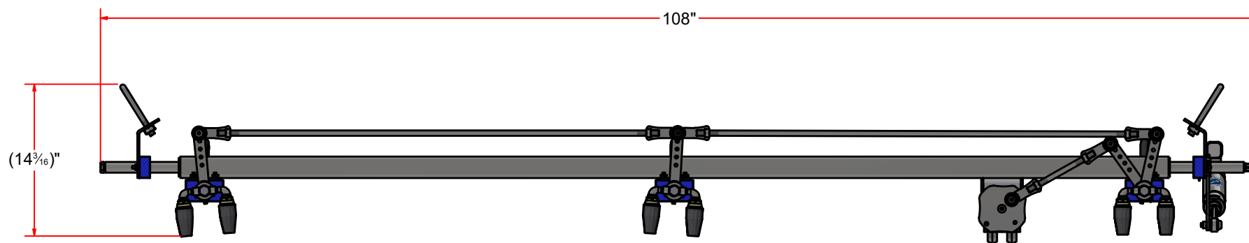
FRONT
