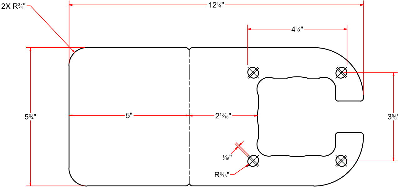
FLAT PATTERN
