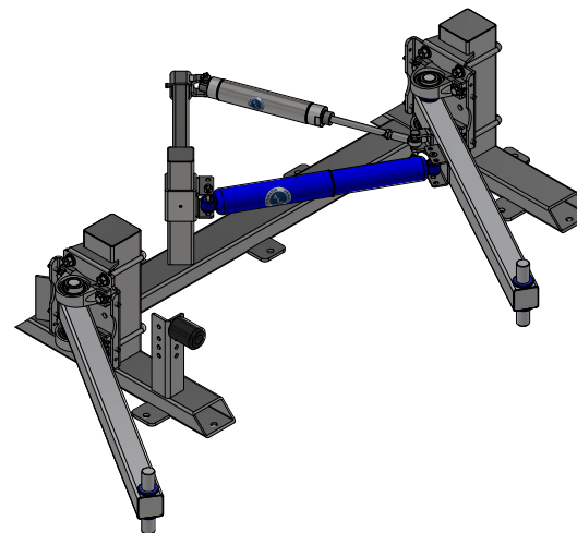
TB3BB - Tire Dressing Frame Assembly [Passenger]
