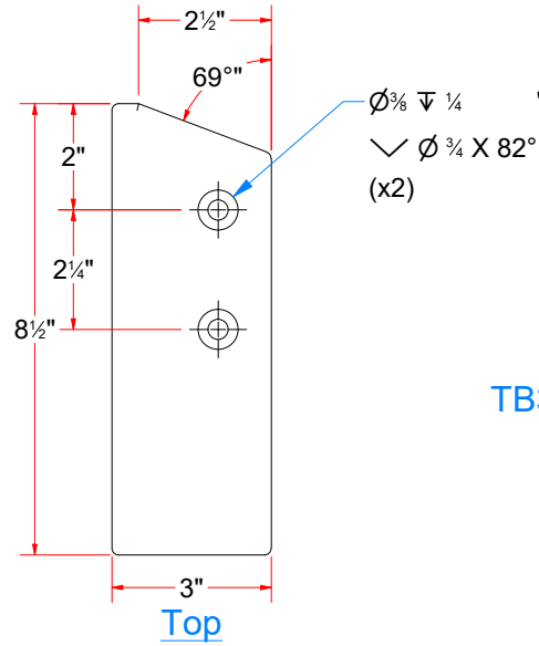
TB3AAAC - Top Plastic Cover [Driver]
