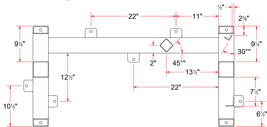
TB3ABA - Tire Shine Frame [Driver]
