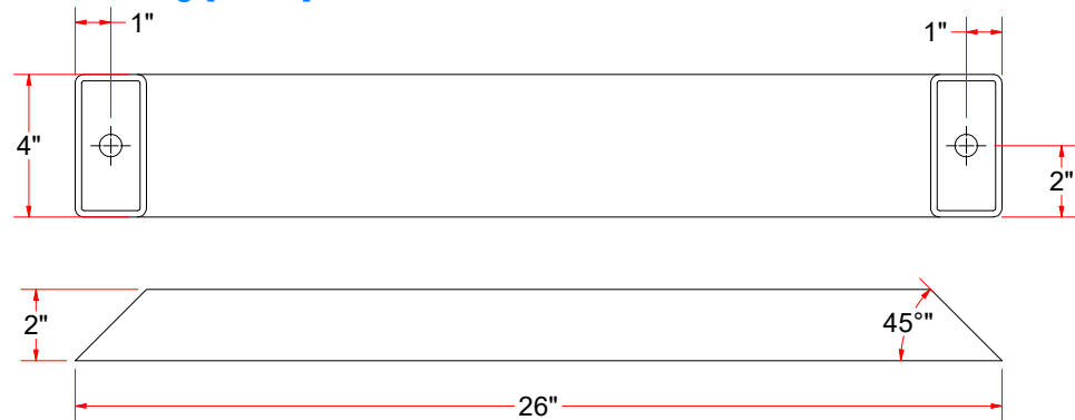
Rct.Tubing [7 Ga.] 2" x 4" x 26" LG
