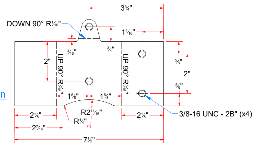
TB3AABBA-EL - Bracket For Motor Mount Plate Assembly
