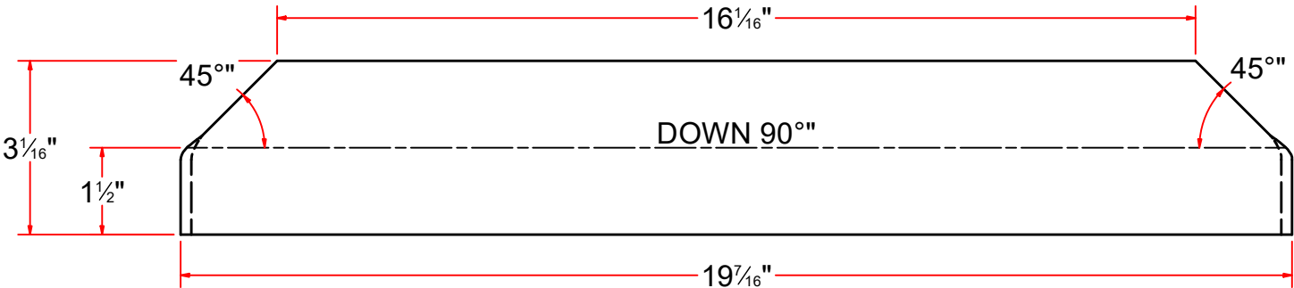
FLAT PATTERN
