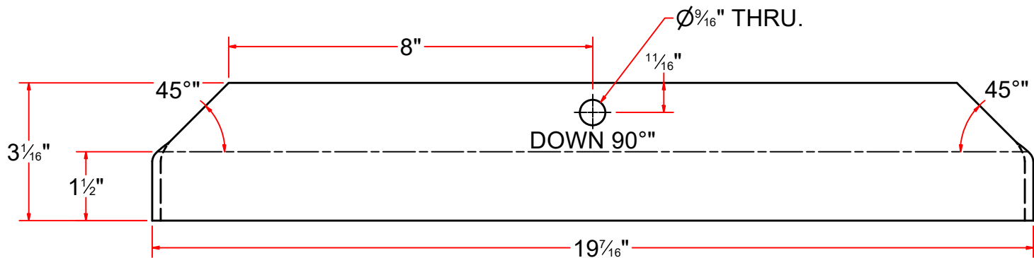
FLAT PATTERN
