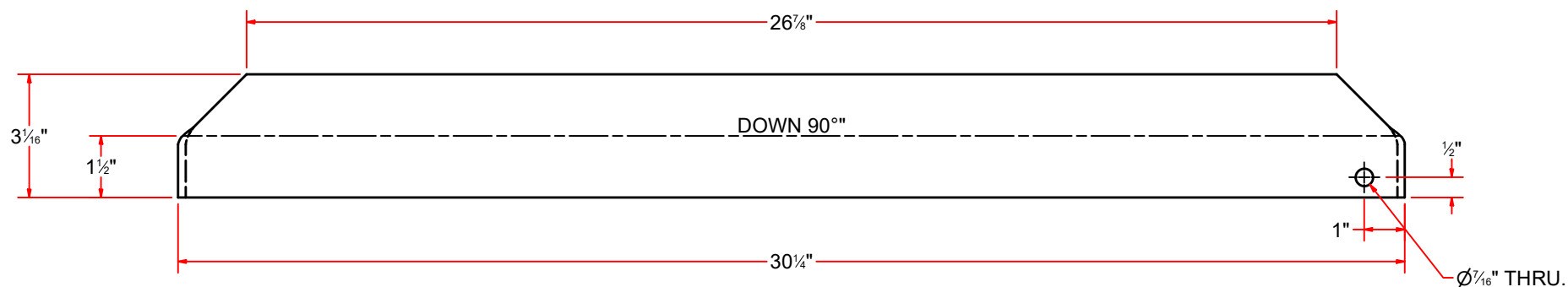
FLAT PATTERN
