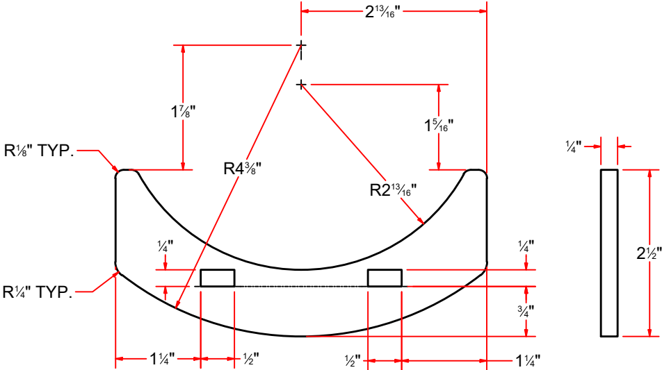
SCALE 1 / 2
