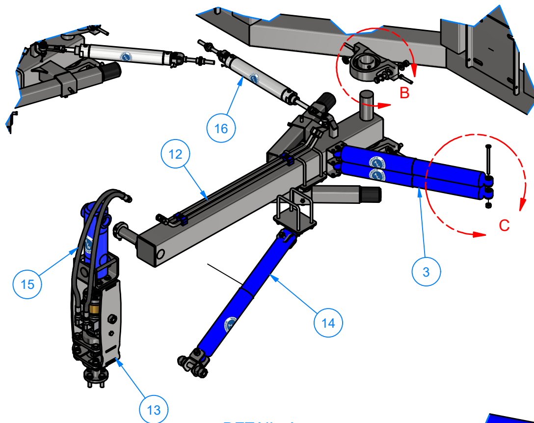
DETAIL A
