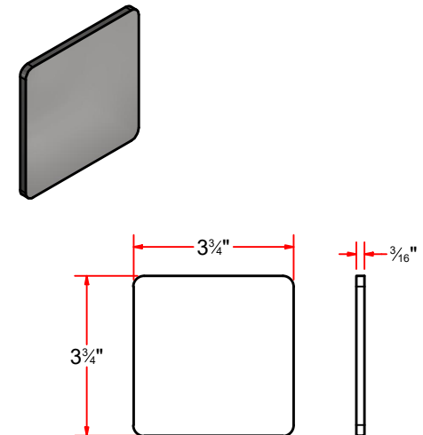
PLSS187X0375X0375X0H - Plate #3/16"x 3 3/4"x 3 3/4"
