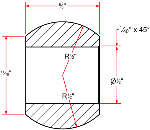
SECTION AC-AC SCALE 2 : 1
