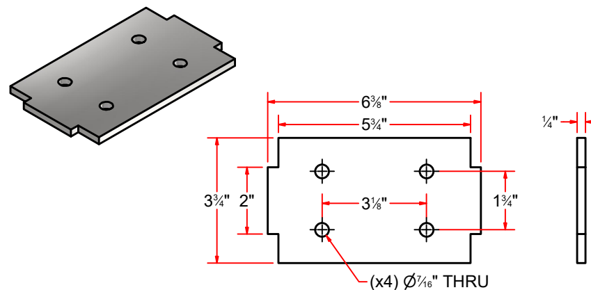
WA10KAA - Plate #1/4" x 3 3/4" x 6 3/8"
