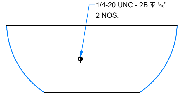
DETAIL M
