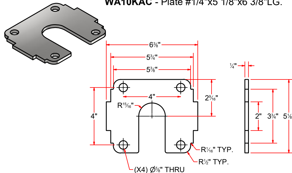
WA10KAC - Plate #1/4"x5 1/8"x6 3/8"LG.
